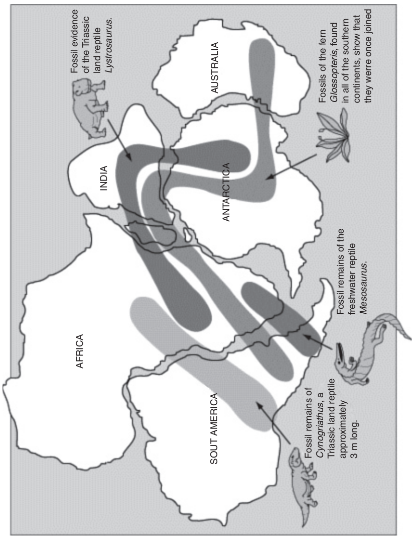
FIGURE 8.3. This map shows how fossil evidence supports the explanation of plate tectonics.
